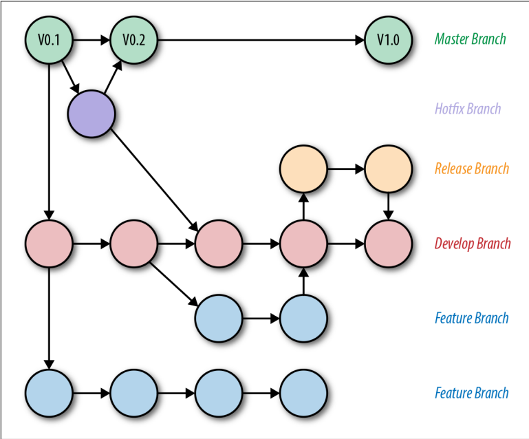
Figure 1-4. Gitflow workflow
