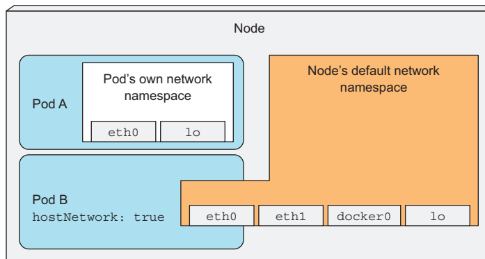
Figure 13.1 A pod with hostNetwork: true uses the node's network interfaces instead of its own.
