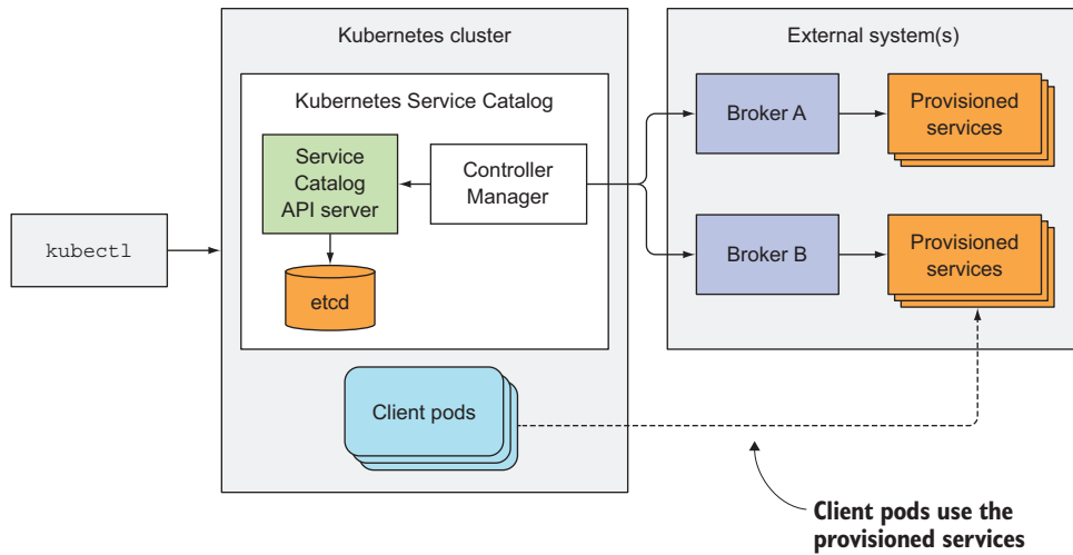
Figure 18.7 The architecture of the Service Catalog
