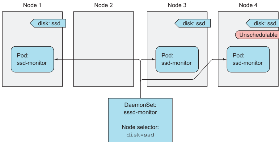
Figure 4.9 Using a DaemonSet with a node selector to deploy system pods only on certain nodes
